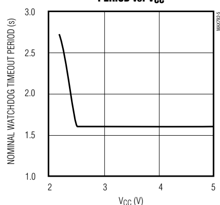
NOMINAL WATCHDOG TIMEOUT PERIOD vs. VCC
