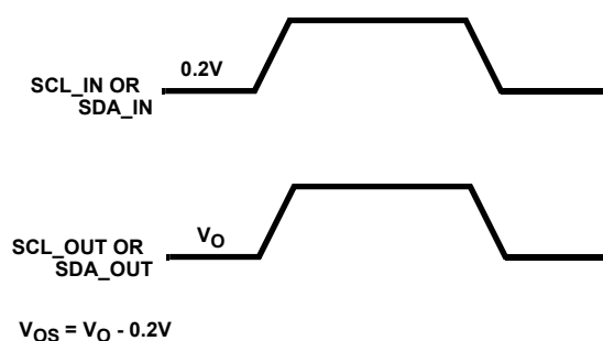
FIGURE 5. INPUT TO OUTPUT OFFSET VOLTAGE
