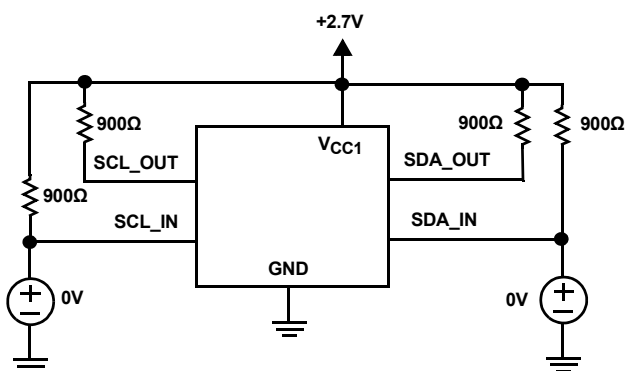
FIGURE 6. OUTPUT LOW VOLTAGE
