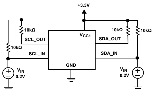
FIGURE 5. INPUT TO OUTPUT OFFSET VOLTAGE
