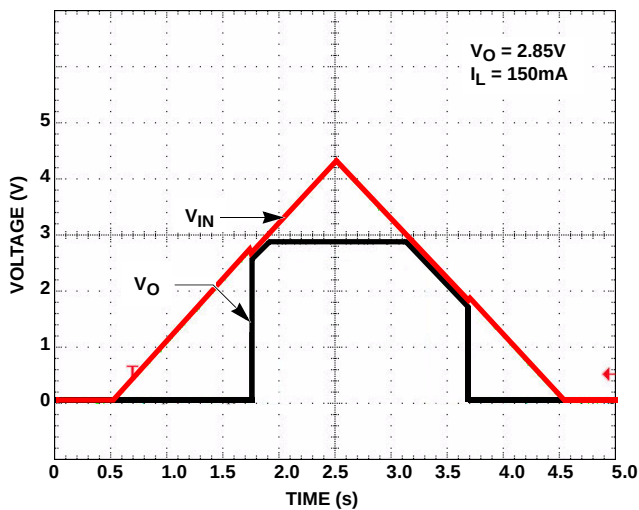
FIGURE 11. POWER-UP/POWER-DOWN
