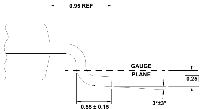
DETAIL "X"
