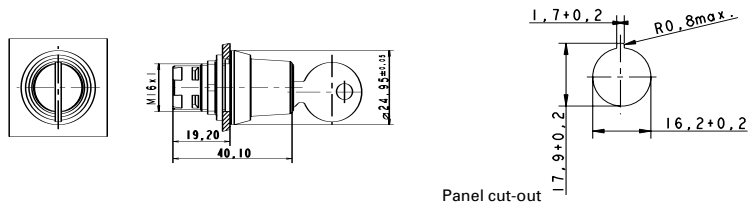
Panel cut-out
