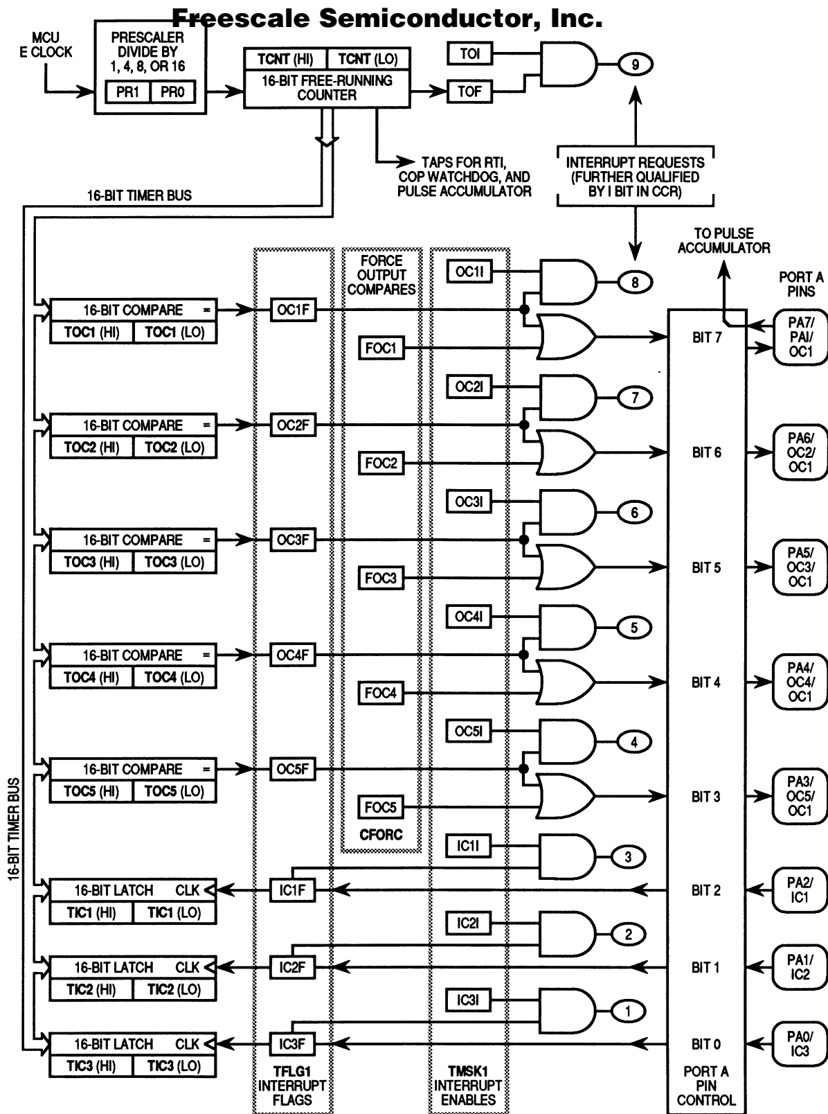
Main Timer
