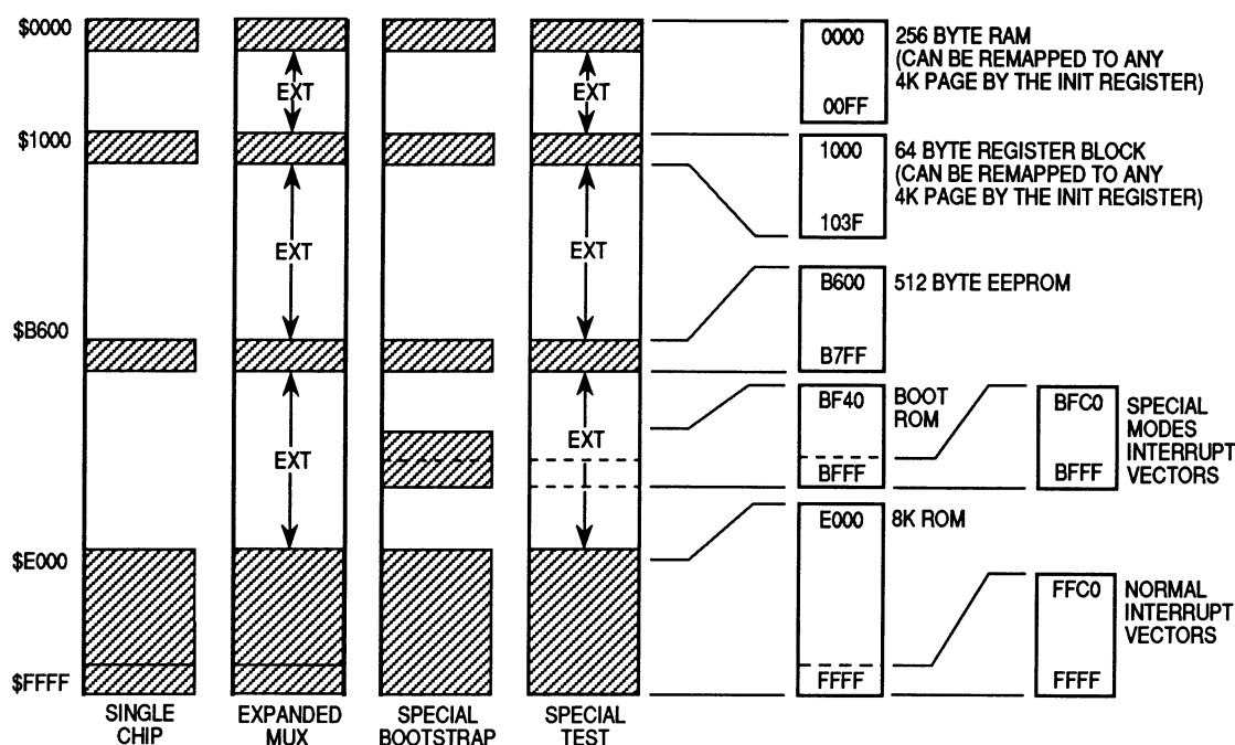
Memory Map
