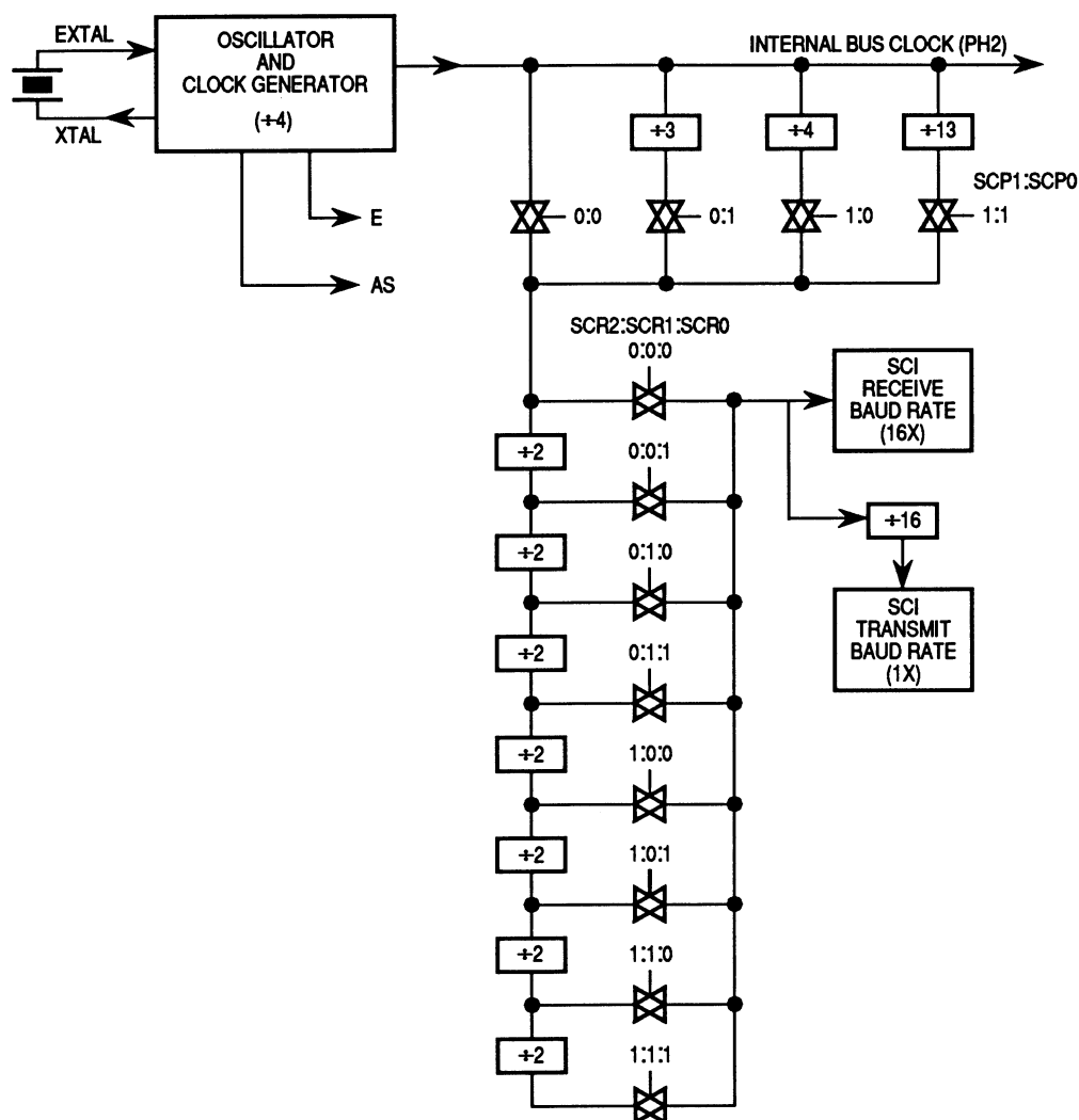
SCI Baud Rate Diagram
