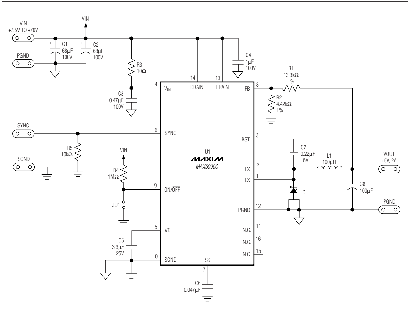
Figure 1. MAX5090 EV Kit Schematic
