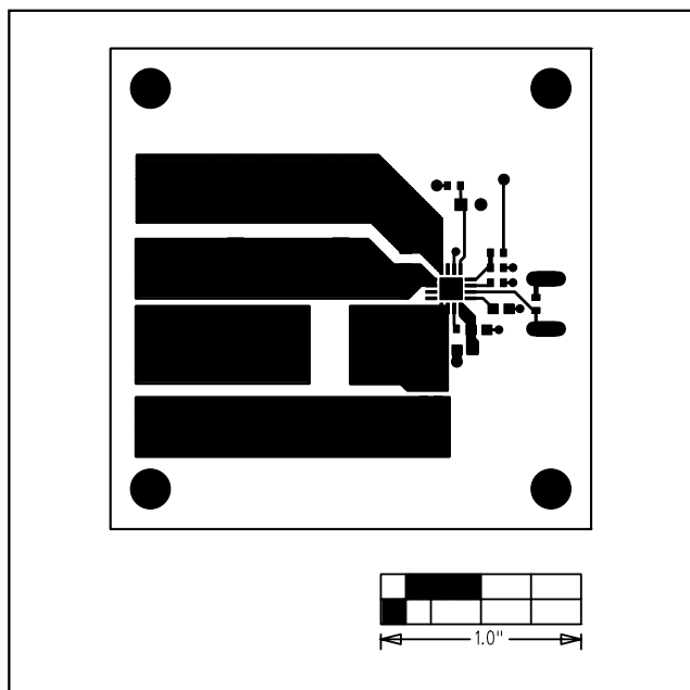
Figure 3. MAX5090 EV Kit PC Board Layout—Component Side
