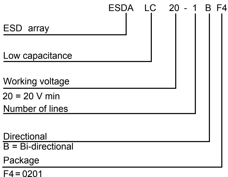
Figure 15. Ordering information scheme
