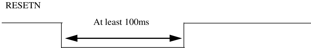
Figure 2. RESETN Timing
