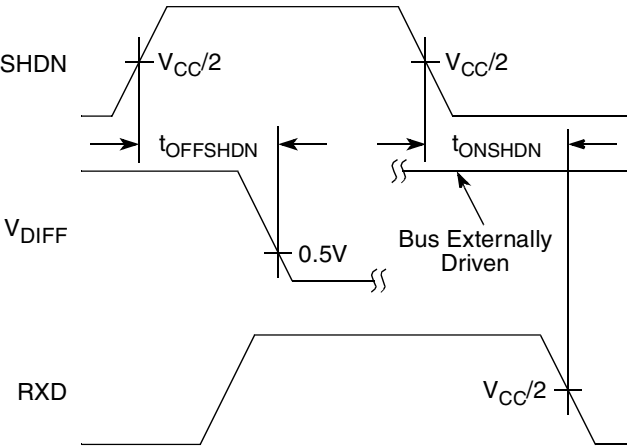
Figure 18. Timing Diagram for FlexCAN Shutdown Signal
