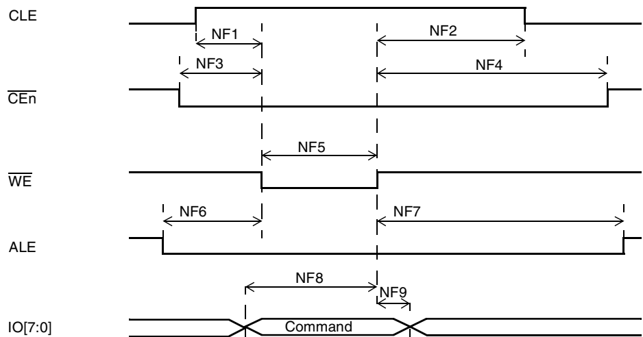
Figure 20. Command Latch Cycle Timing Diagram
