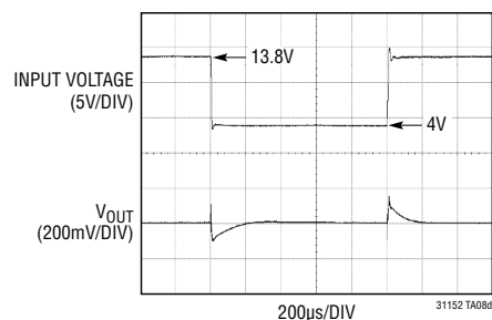
Fast (10 \mu s) Cold Crank Line Transient, V_{IN} = 13.8V to 4V
