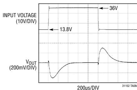
Fast (10μs) Load Dump Line Transient, V_{IN} = 13.8V to 36V
