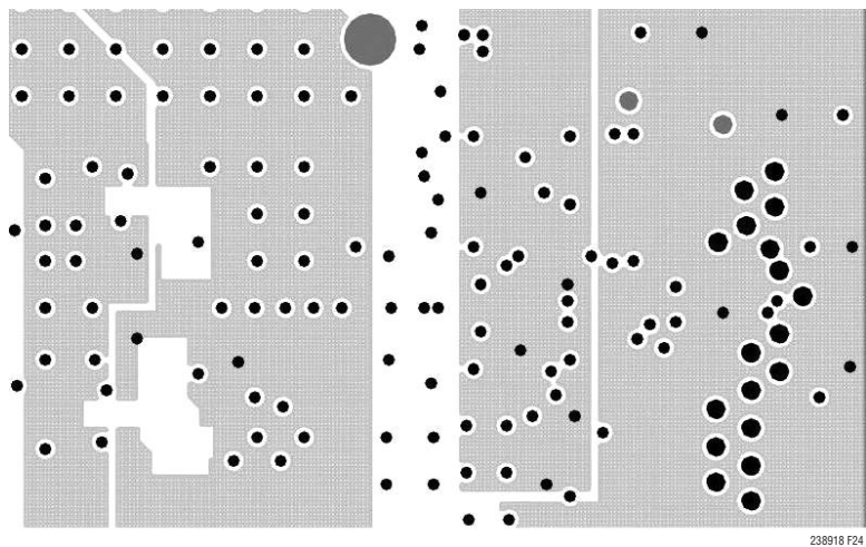
Partial Layer 3 Power Plane
