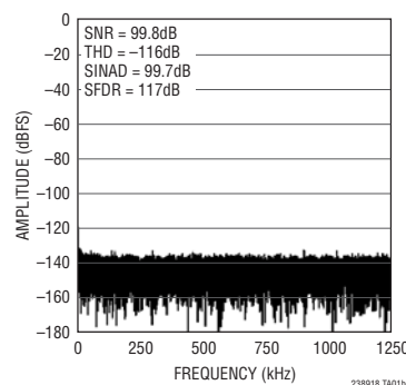
32k Point FFT f_{\text{SAMPL}} = 2.5\text{Mpsps} , f_{\text{IN}} = 2\text{kHz}
