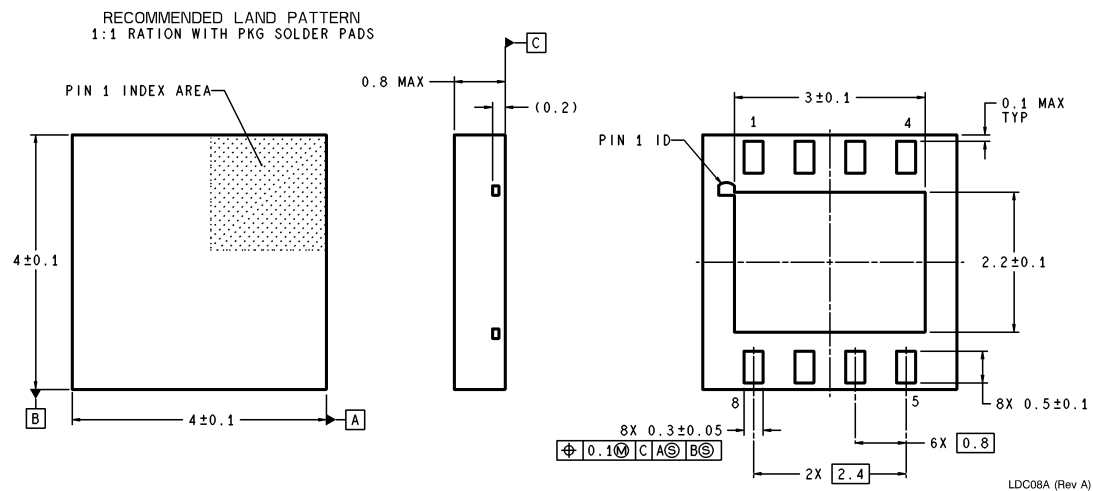
8-Lead LLP NS Package Number LDC08A
