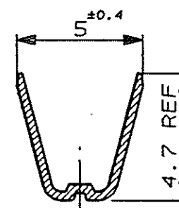
SECT B-B
