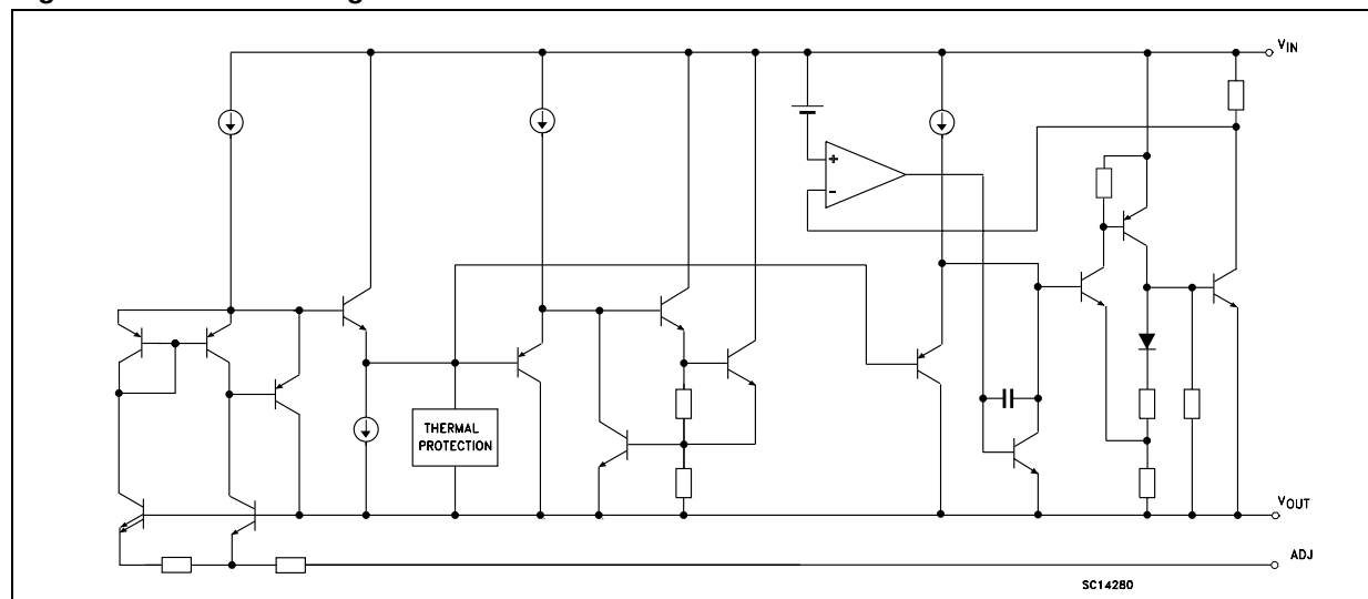
Figure 1: Schematic Diagram
