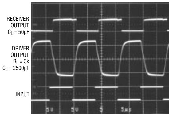
Output Waveforms
