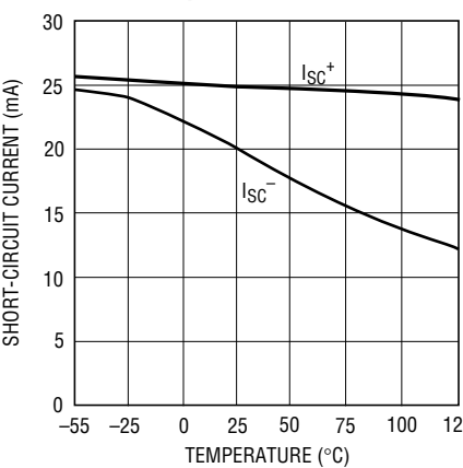
Driver Output Short-Circuit Current
