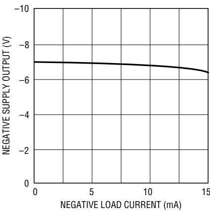
Negative Supply Output Compliance Curve
