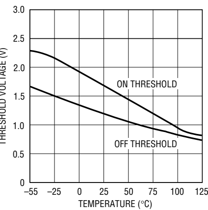
On/Off Thresholds
