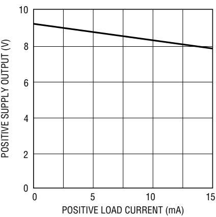
Positive Supply Output Compliance Curve
