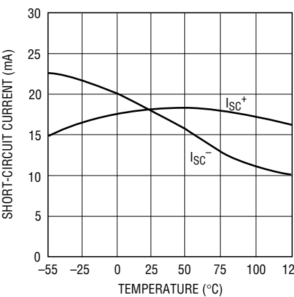
Receiver Short-Circuit Current
