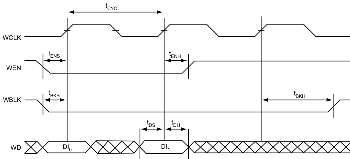
Figure 2-37 • FIFO Write
