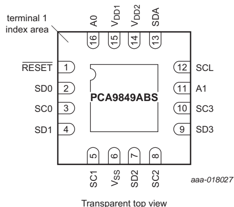
Fig 3. Pin configuration for HVQFN16
