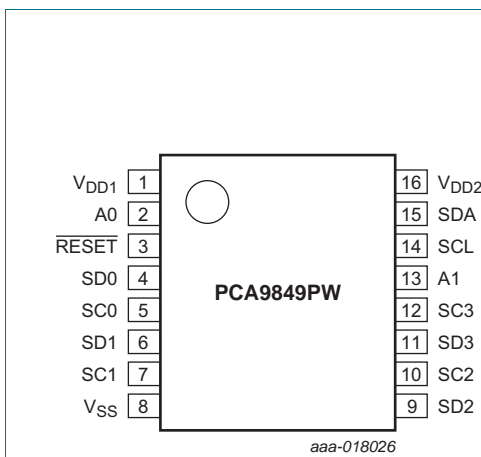
Fig 2. Pin configuration for TSSOP16
