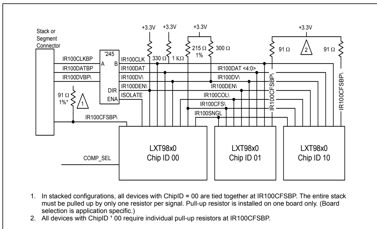
Figure 30 Typical 100 Mbps IRB Implementation
