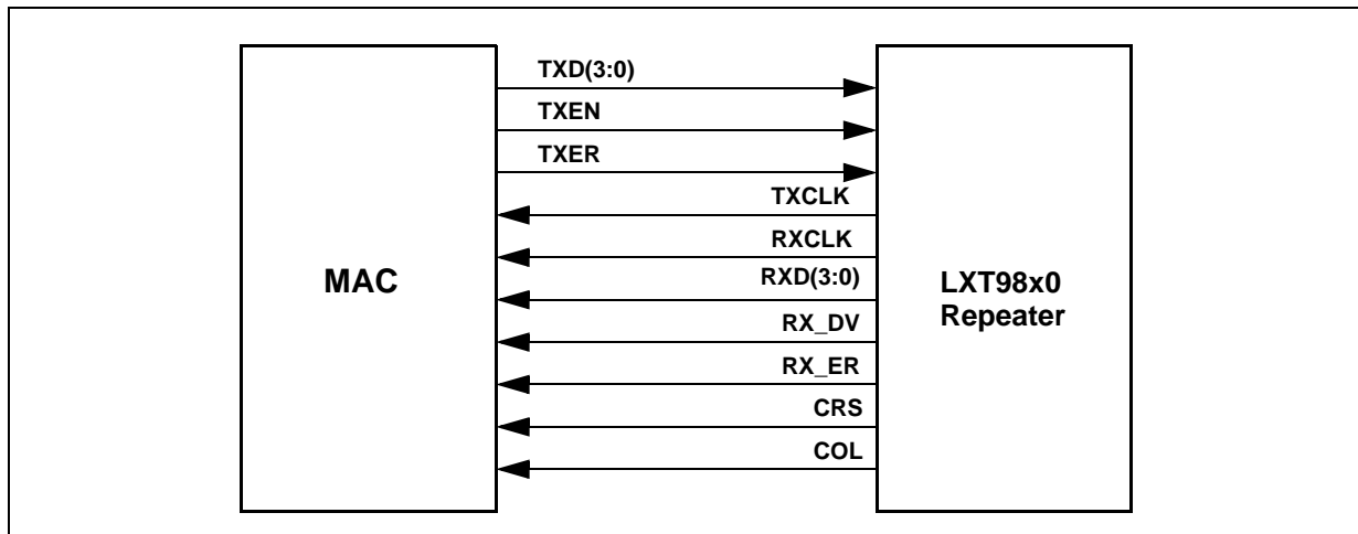
Figure 4 MII Interface
