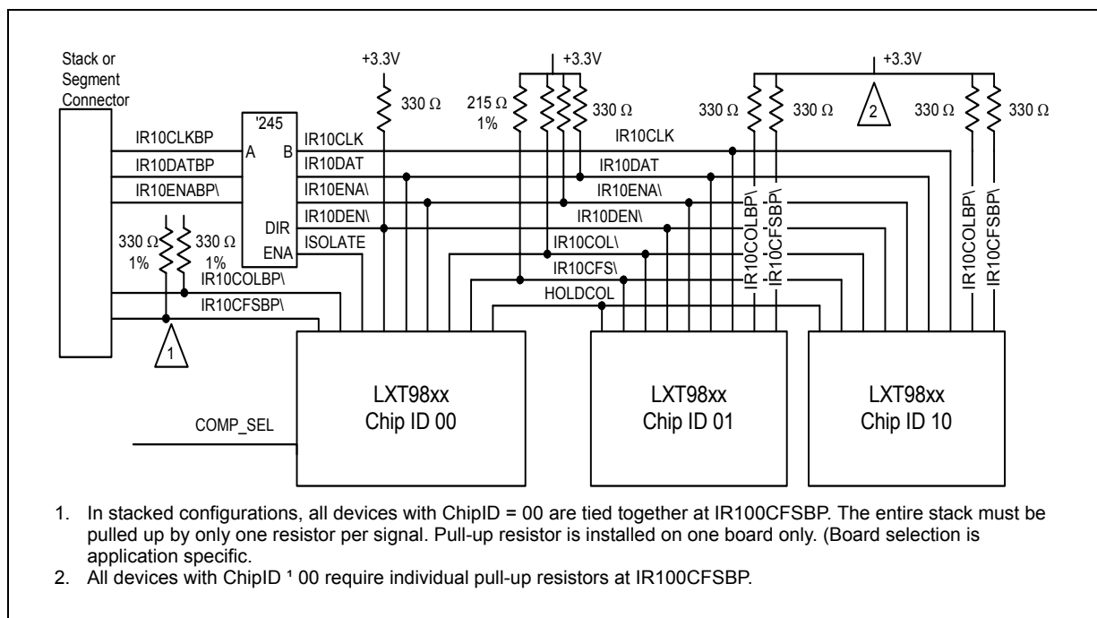
Figure 31 Typical 10 Mbps IRB Implementation
