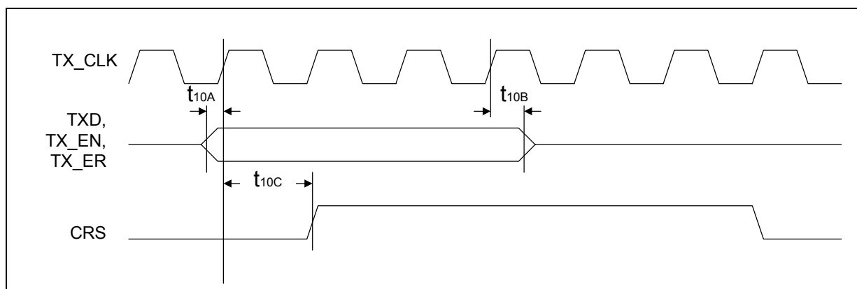
Figure 35 10BASE-T MII-to-TP Timing
