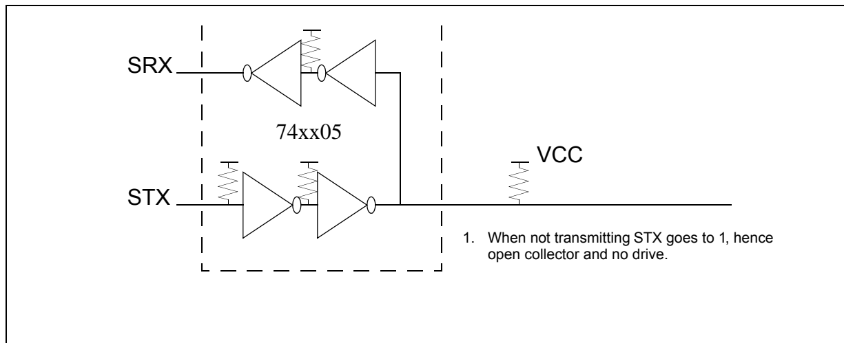
Figure 23 Typical Serial Management Interface Connections
