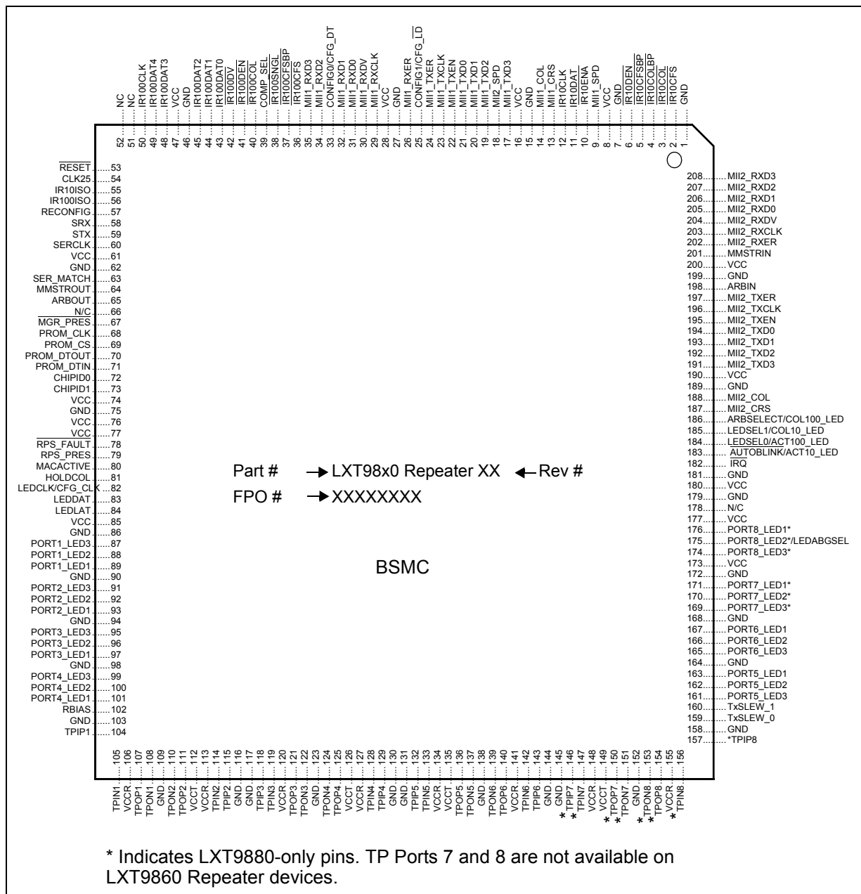
Figure 2 Pin Assignments
