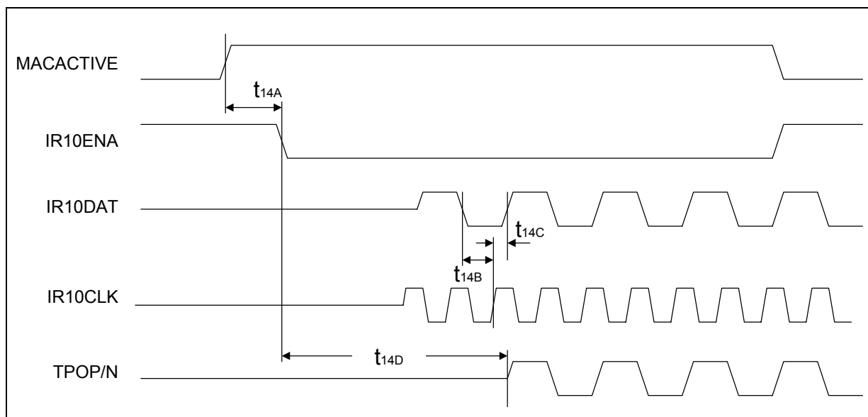
Figure 39 10 Mbps IRB-to-TP Port Timing
