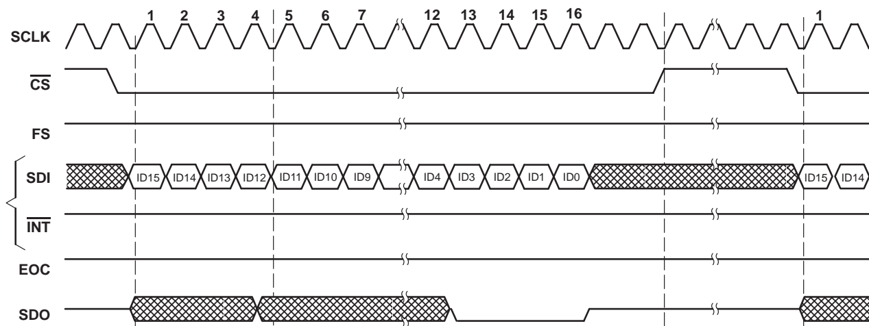
Figure 6. TLC2554/TLC2558 Write Cycle ( \overline{\text{FS}} = 1 )
