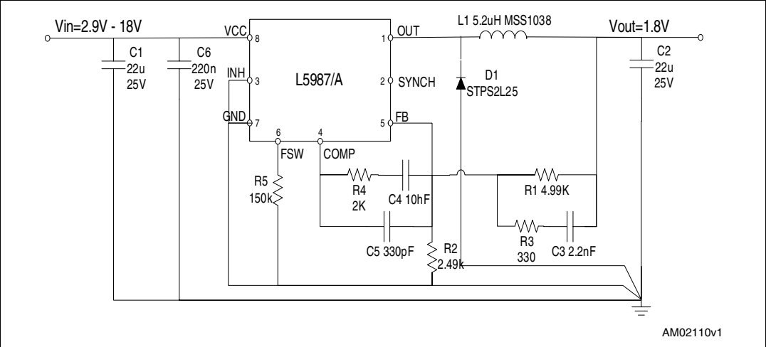
Figure 1. Application circuit
