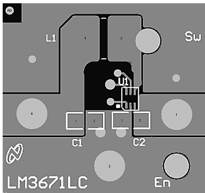
Figure 9. Top Layer (6-pin USON)
