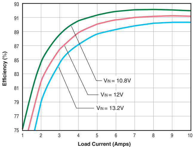
LSM-2/10-D12 Efficiency vs. Line Voltage and Load Current @ +25°C
