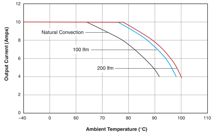
LSM-1.2/10-D12 Maximum Output Current vs. Ambient Temperature (SMT mount, air flow direction from pin 2 to pin 1)
