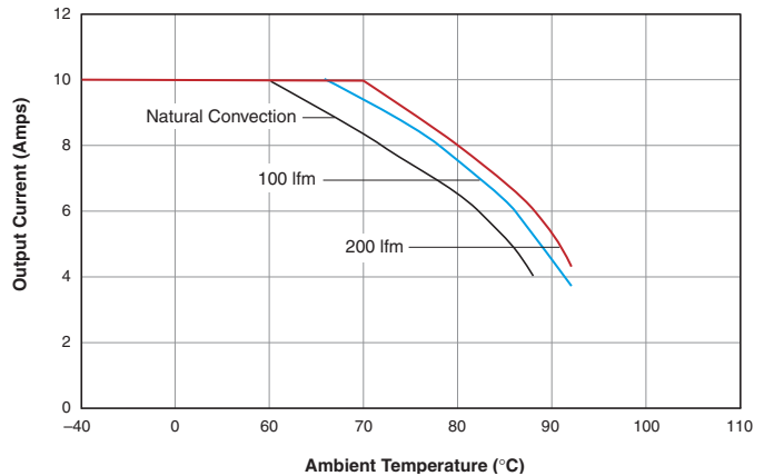
LSM-1.5/10-D12 Maximum Output Current vs. Ambient Temperature (SMTmount, air flow direction from pin 2 to pin 1)
