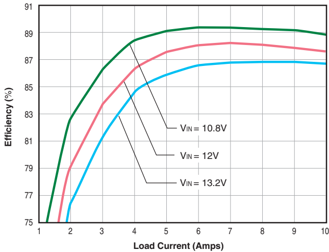
LSM-1.2/10-D12 Efficiency vs. Line Voltage and Load Current @ +25°C
