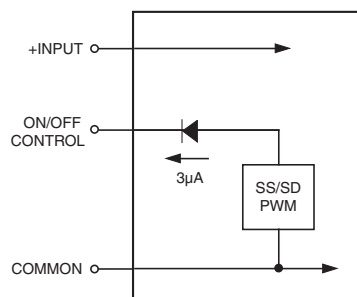
Figure 4A. LSM-T10-D12 Driving the On/Off Control Input
