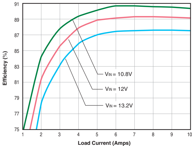
LSM-1.5/10-D12 Efficiency vs. Line Voltage and Load Current @ +25°C
