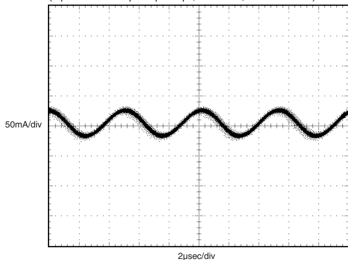
Input Reflected Ripple Current
