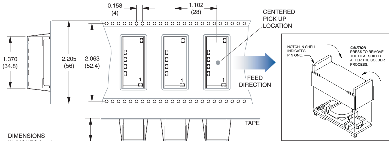
Figure 7. Tape Dimensions
