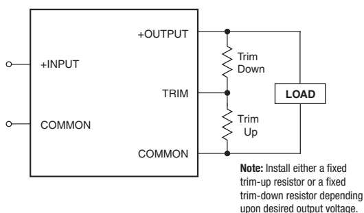
Figure 7. Trim Connections Using Fixed Resistors
