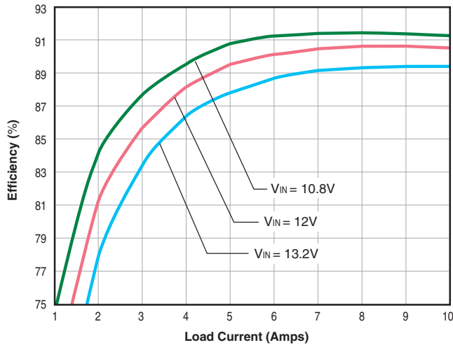
LSM-1.8/10-D12 Efficiency vs. Line Voltage and Load Current @ +25°C
