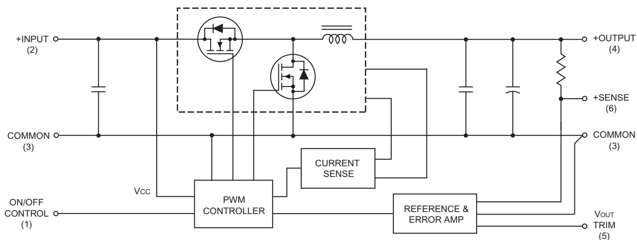
Figure 1. Simplified Schematic
