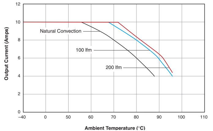
LSM-2/10-D12 Maximum Output Current vs. Ambient Temperature (SMT mount, air flow direction from pin 2 to pin 1)
