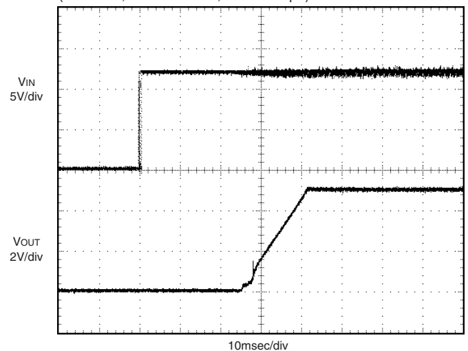
Start-Up from ON/OFF
