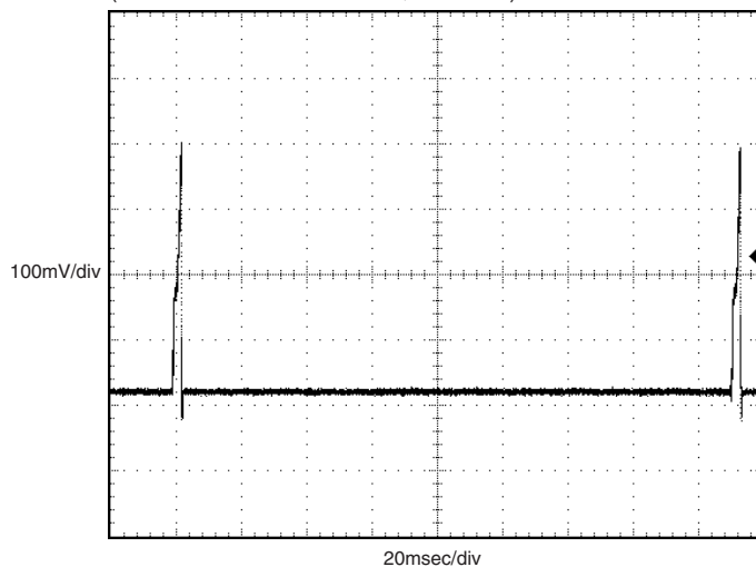
Output Hiccup
