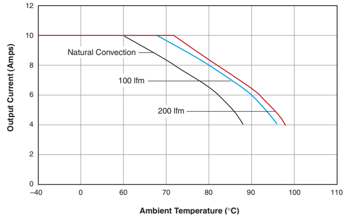
LSM-1.8/10-D12 Maximum Output Current vs. Ambient Temperature (SMT mount, air flow direction from pin 2 to pin 1)
