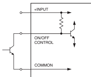
Figure 4. Driving the On/Off Control Pin with an Open-Collector Drive Circuit (All models except LSM-T/10-D12)
