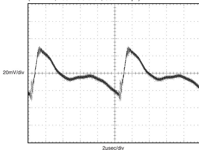
Output Ripple and Noise
