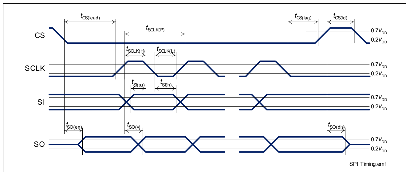
Figure 20 Timing Diagram SPI Access
