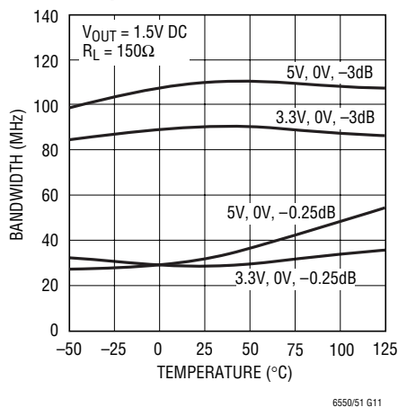
-3dB, -0.25dB Bandwidth vs Temperature
