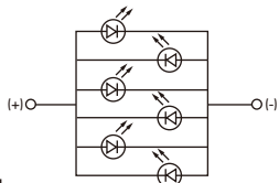
AT621 Bicolor LED 5-volt 6-element with Resistor
