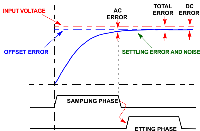
FIGURE 26. INPUT SAMPLING OPERATION
