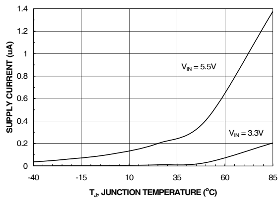
Figure 6. Reverse Current vs. Temperature
