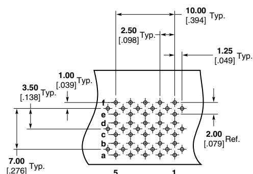
Coplanar Daughtercards (Pin 1a Header = Pin 5a Shroud Side) Recommended PC Board Layout — Reference Page 60 (Shroud Side Shown)
