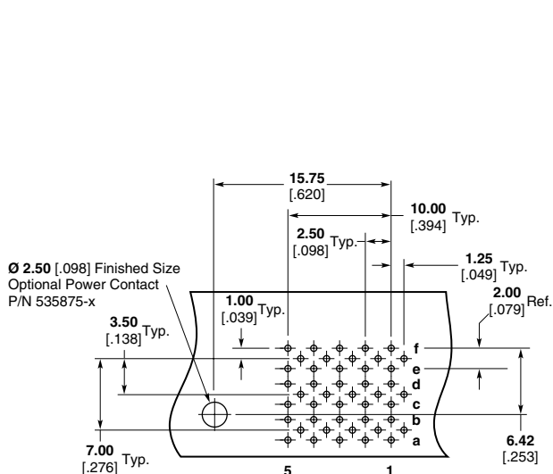
Recommended PC Board Layout (Component Side Shown) For Non-Midplane Applications For Midplane Applications Reference Page 60
