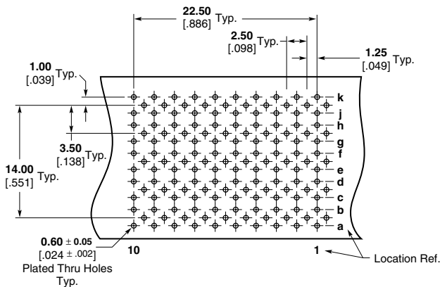
Non-Coplanar Daughtercards (Pin 1a Header = Pin 1k Shroud Side) Recommended PC Board Layout — Reference Page 74 (Shroud Side Shown)
