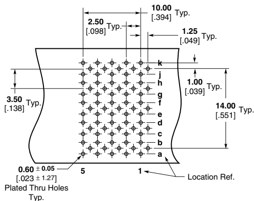
Non-Coplanar Daughtercards (Pin 1a Header = Pin 1k Shroud Side) Recommended PC Board Layout — Reference Page 74 (Shroud Side Shown)
