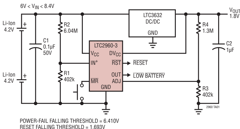
Battery and Regulator Monitor
