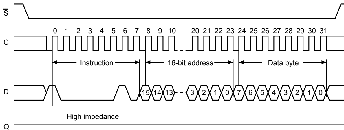
Figure 18. Lock ID sequence
