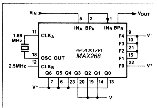
Figure 20. 4th-Order 50kHz Chebyshev Bandpass Using No External Resistors
