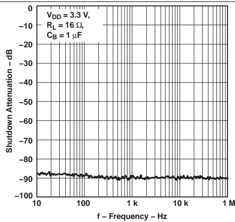
Figure 25. Shutdown Attenuation vs Frequency
