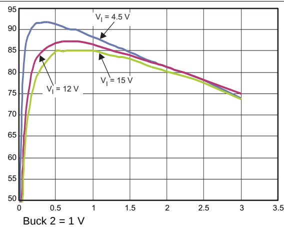
Figure 4. Efficiency
