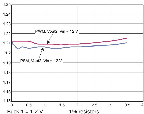
Figure 2. Load Regulation
