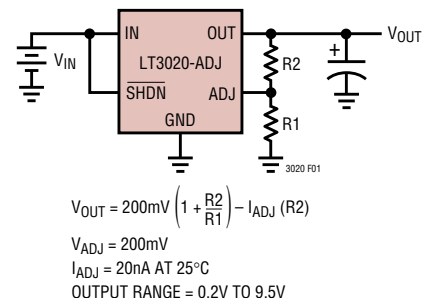
Figure 1. Adjustable Operation
