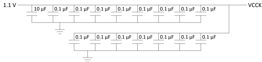
Figure 8-2. VCCCK Recommended Filter
