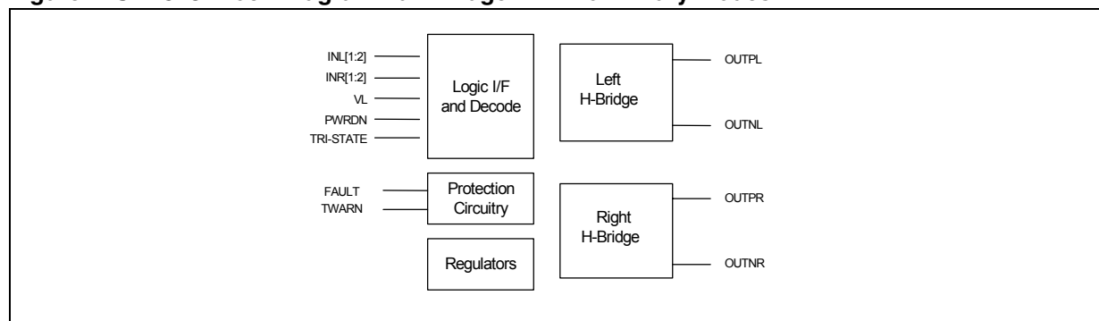
Figure 7. STA518 Block Diagram Full-Bridge DDX® or Binary Modes
