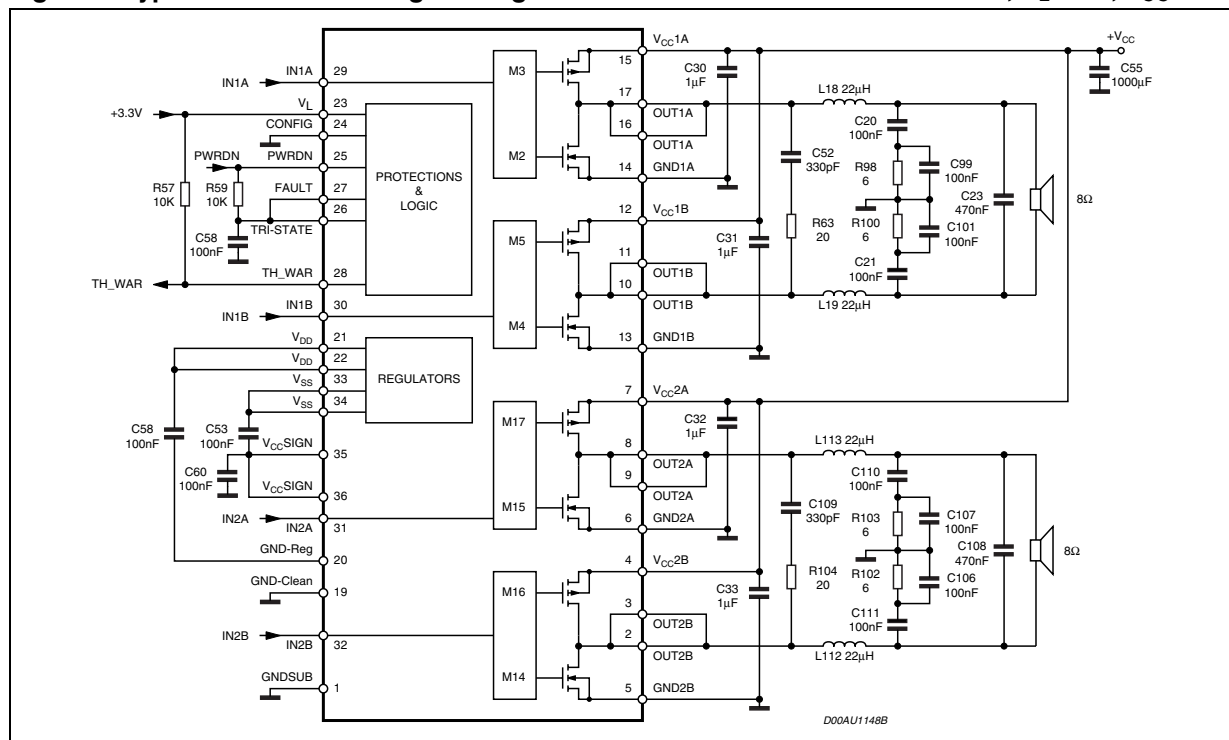
Figure 9. Typical Stereo Full Bridge Configuration to Obtain 50+50W @ THD = 10%, R_L = 8\Omega , V_{CC} = 29V
