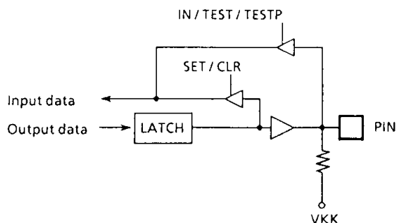
Figure2-3. Ports R3, RA, RB, RC
