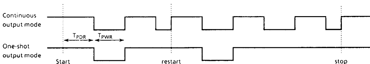
Figure 2-8. Internal clock mode
