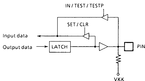
Figure 2-2. Ports R1, R2
