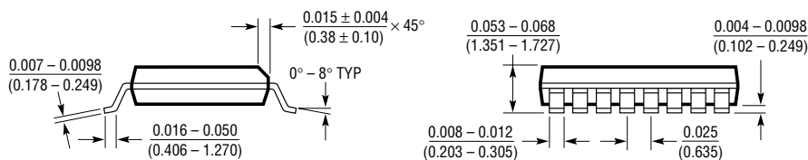
GN Package 16-Lead Plastic SSOP (Narrow 0.150) (LTC DWG # 05-08-1641)
