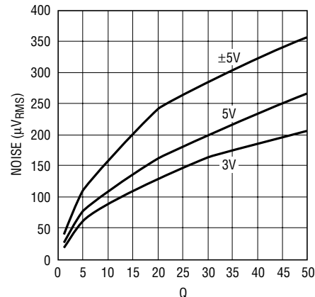
LTC1067-50 Noise vs Q
