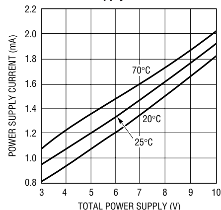
LTC1067-50 Power Supply Current vs Power Supply
