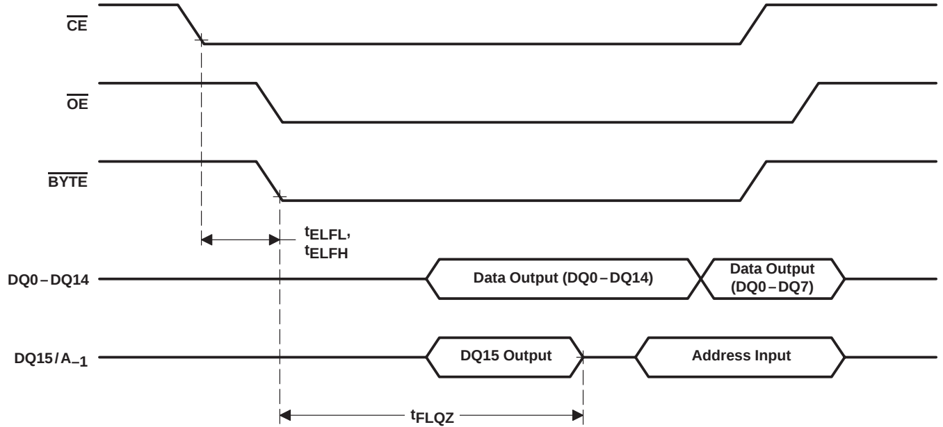
Figure 26. \overline{\text{BYTE}} Timing Diagram for Read Operation
