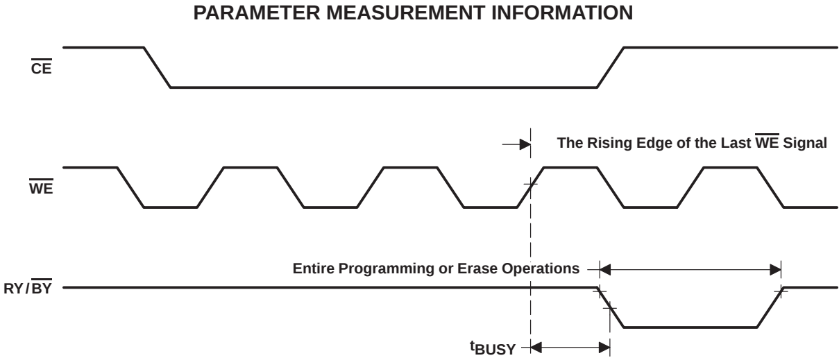
Figure 28. \overline{RY}/\overline{BY} Timing Diagram During Program/Erase Operations
