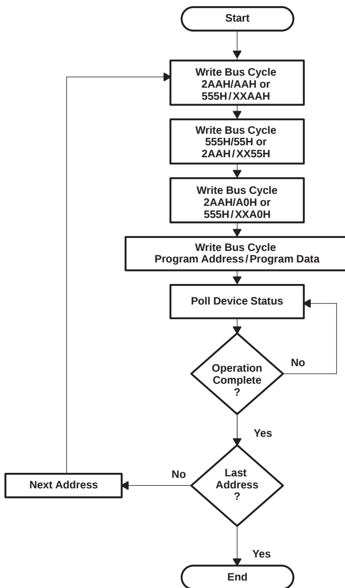
Figure 9. Program Algorithm
