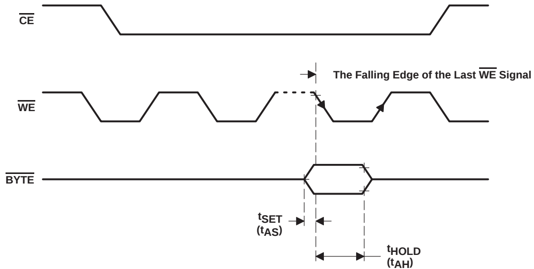
Figure 27. \overline{\text{BYTE}} Timing Diagram for Write Operation
