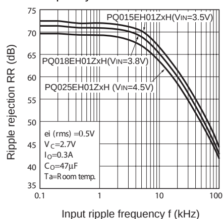
Fig.18 Ripple Rejection vs. Input Ripple Frequency
