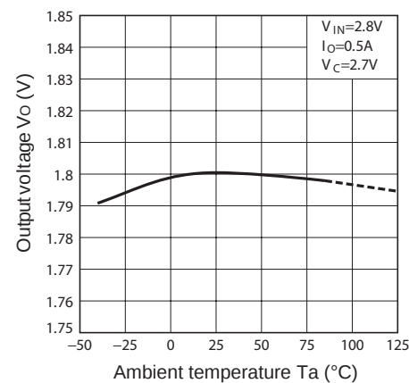
Fig.8 Output Voltage vs. Ambient Temperature (PQ018EH01ZxH)
