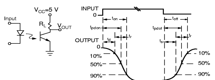
Figure 8. Switching time test schematic and waveform
