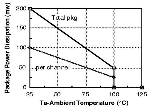
Figure 7. Power dissipation versus ambient temperature
