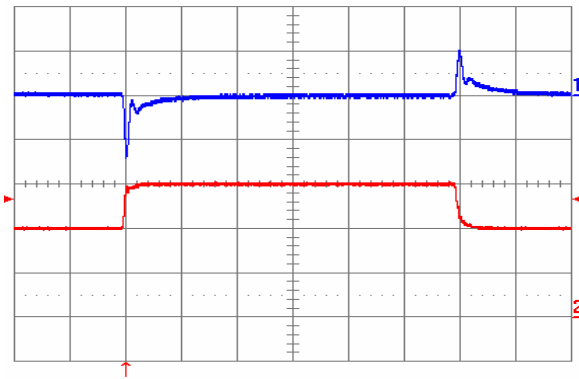
Fig. 1.2V.9: Output voltage response to load current step-change (20 A – 30 A – 20 A) at V_{in} = 48 V. Top trace: output voltage (100 mV/div.). Bottom trace: load current (10 A/div). Current slew rate: 1 A/ \mu s. C_o = 470 \mu F tantalum + 1 \mu F ceramic. Time scale: 0.2 ms/div.
