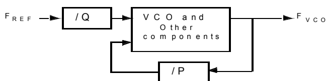
Figure 4. PLL system
