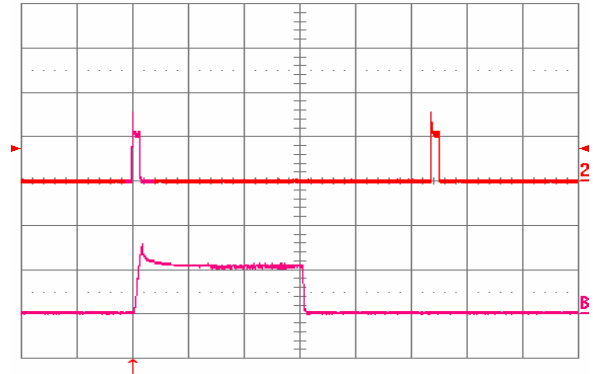
Fig. 27: Load current (top trace, 10 A/div, 20 ms/div) into a 10 mΩ short circuit during restart, at Vin = 48 V. Bottom trace (10 A/div, 1 ms/div) is an expansion of the on-time portion of the top trace.
