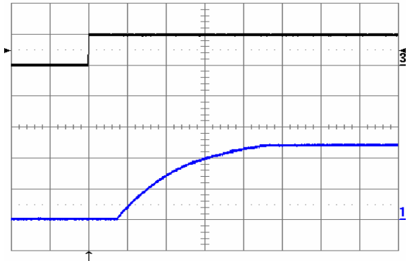
Fig. 19: Turn-on transient at full rated load current (resistive) plus 2,200 \mu\text{F} at V_{in} = 48\text{ V} , triggered via ON/OFF pin. Top trace: ON/OFF signal (5 V/div.). Bottom trace: output voltage (5 V/div.). Time scale: 2 ms/div.
