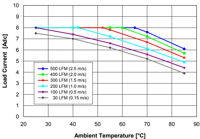
Fig. 1: Available load current vs. ambient air temperature and air-flow rates for Q48T08120 converter mounted vertically with air flowing from pin 3 to pin 1, MOSFET temperature \leq 120^{\circ}\text{C} , V_{in} = 54\text{ V} .
