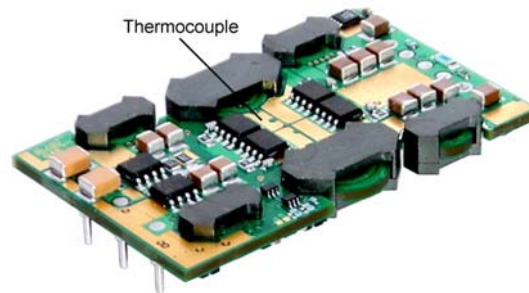
Fig. 28: Location of the thermocouple for thermal testing.
