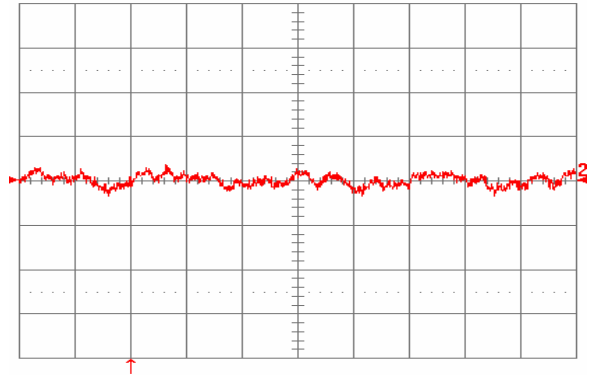
Fig. 25: Input reflected ripple current, i_s (10 mA/div.), measured through 10 \mu\text{H} at the source at full rated load current and V_{in} = 48 \text{ V} . Refer to Fig. 23 for test setup. Time scale: 1 \mu\text{s}/\text{div} .
