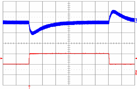
Fig. 20: Output voltage response to load current step-change (2 A – 4 A – 2 A) at V_{in} = 48\text{ V} . Top trace: output voltage (200 mV/div.). Bottom trace: load current (2 A/div.). Current slew rate: 0.1 A/ \mu\text{s} . C_o = 1\text{ }\mu\text{F} ceramic. Time scale: 0.5 ms/div.
