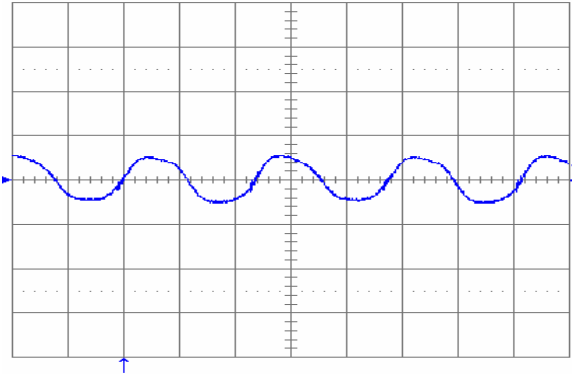
Fig. 22: Output voltage ripple (50 mV/div.) at full rated load current into a resistive load with C_o = 10 \mu\text{F} tantalum + 1\mu\text{F} ceramic and V_{in} = 48 \text{ V} . Time scale: 1 \mu\text{s}/\text{div} .
