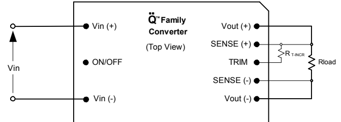
Fig. 4: Configuration for increasing output voltage.
