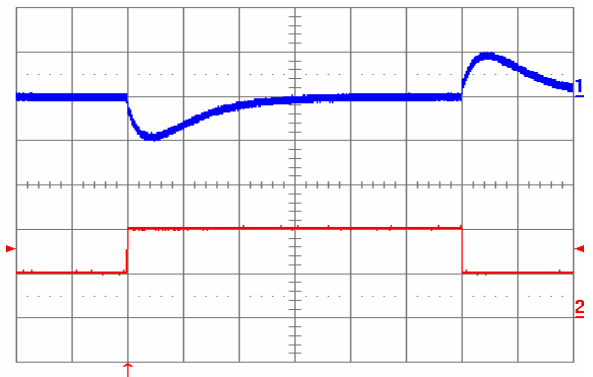
Fig. 21: Output voltage response to load current step-change (2 A – 4 A – 2 A) at V_{in} = 48\text{ V} . Top trace: output voltage (200 mV/div.). Bottom trace: load current (2 A/div.). Current slew rate: 5 A/ \mu\text{s} . C_o = 450\text{ }\mu\text{F} tantalum + 1 \mu\text{F} ceramic. Time scale: 0.5 ms/div.
