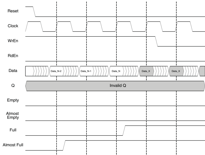
Figure 11-22. FIFO without Output Registers, End of Data Write Cycle
