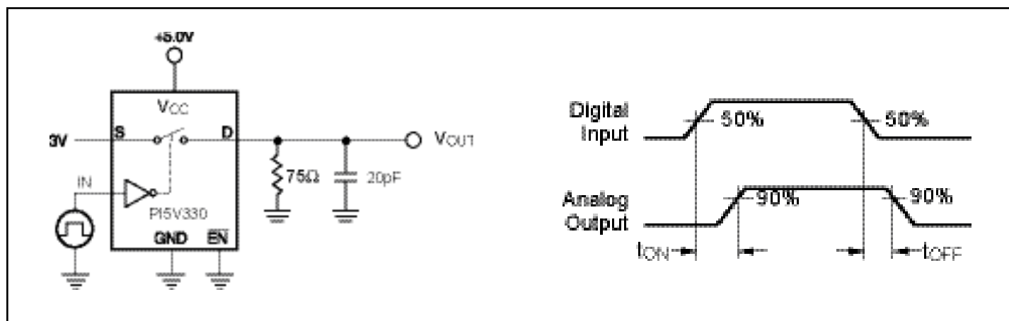
Figure 4. Switching Time
