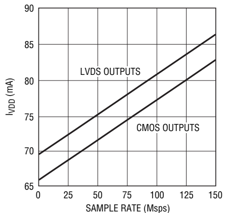
LTC2262-12: I_{VDD} vs Sample Rate, 5MHz Sine Wave Input, -1dB
