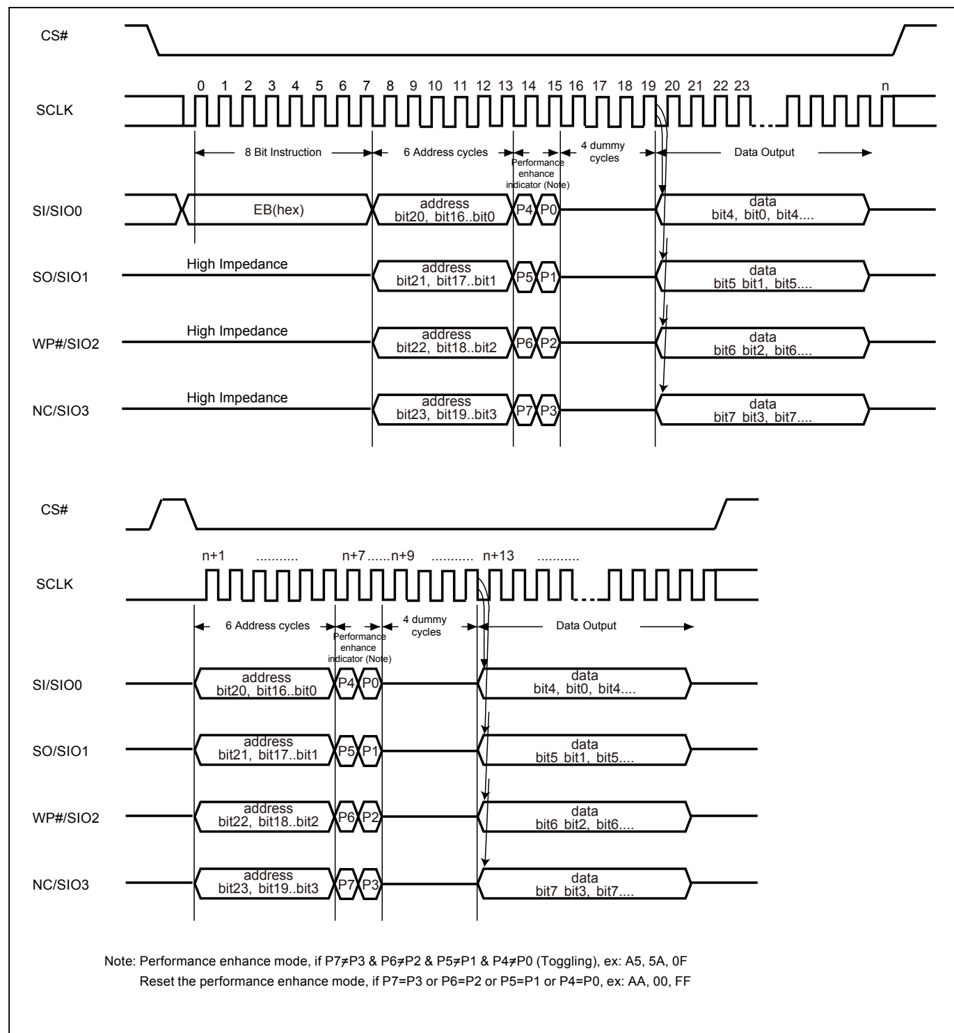
Figure 21. 4 x I/O Read enhance performance Mode Sequence (Command EB)
