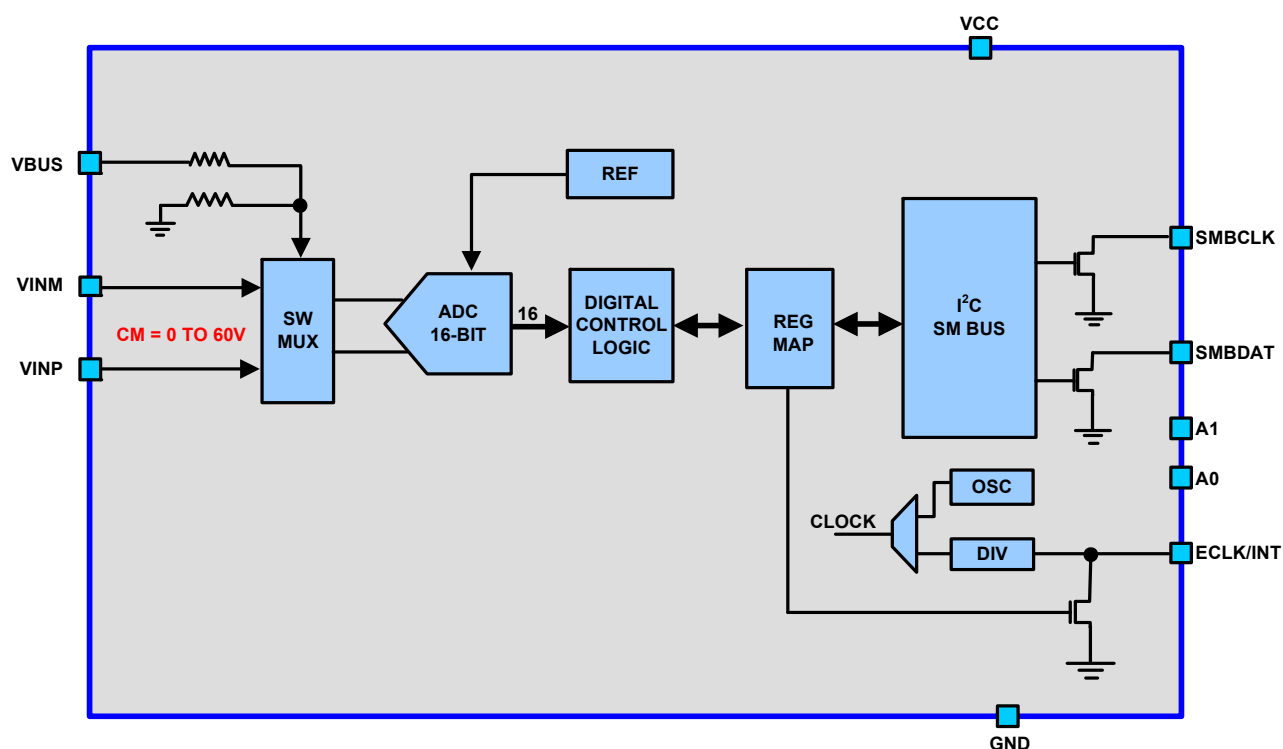
FIGURE 2. BLOCK DIAGRAM
