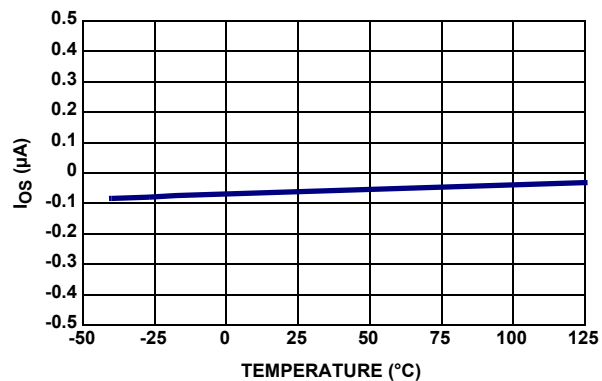
FIGURE 20. SHUNT I_{OS} vs TEMPERATURE (MODE 5)
