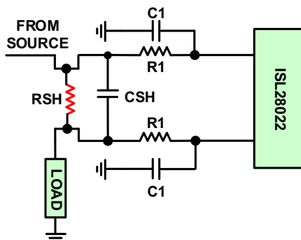
FIGURE 35. SIMPLIFIED FILTER DESIGN TO IMPROVE NOISE PERFORMANCE TO THE ISL28022
