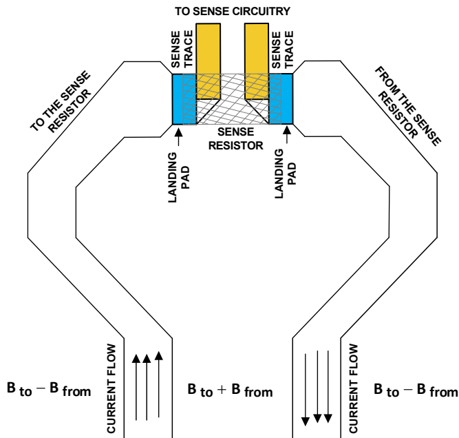
FIGURE 48. CLOSELY ROUTED TRACES THAT CONNECT TO THE SENSE RESISTOR REDUCES THE MAGNETIC INTERFERENCE SOURCED FROM THE CURRENT FLOWING THROUGH THE TRACES
