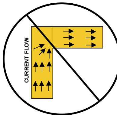
FIGURE 44. AVOID ROUTING ORTHOGONAL CONNECTIONS FOR TRACES THAT HAVE HIGH CURRENT FLOWS
