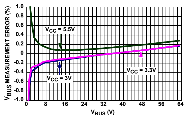
FIGURE 9. V_{BUS} MEASUREMENT ERROR vs V_{BUS} ( T_A = +25^\circ\text{C} )
