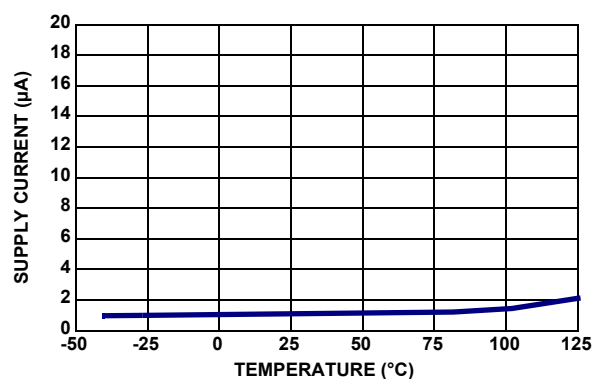
FIGURE 14. SUPPLY CURRENT vs MODE 0 vs TEMPERATURE
