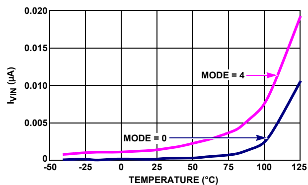
FIGURE 18. SHUNT I_{VIN} vs TEMPERATURE (MODE 0, 4)
