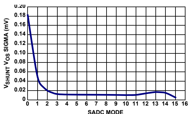
FIGURE 36. MEASUREMENT STABILITY vs SADC MODE
