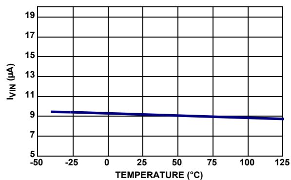
FIGURE 16. SHUNT I_{VIN} vs TEMPERATURE (MODE 5)
