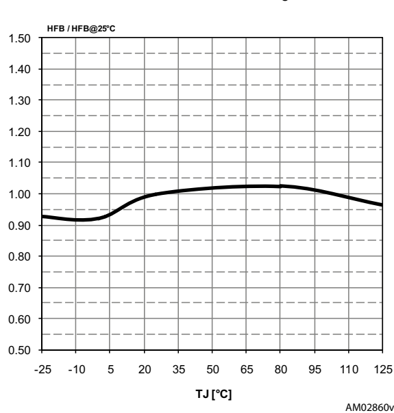
Figure 10. HFB vs. T_J
